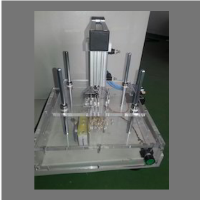
PCB Functional Test Fixture
