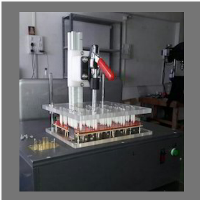
PCB Testing Fixture
