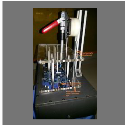
PCB FT Fixture
