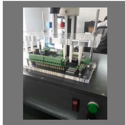
Pcb Testing Jigs
